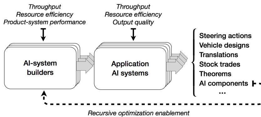
Figure 2: Optimization pressures during AI system development focus resources on tasks and enable further development based on task-focused components.
